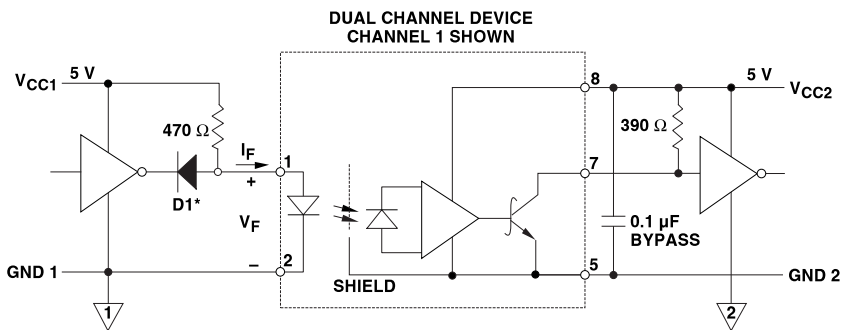
Figure 18. Recommended TTL/LSTTL to TTL/LSTTL interface circuit.
