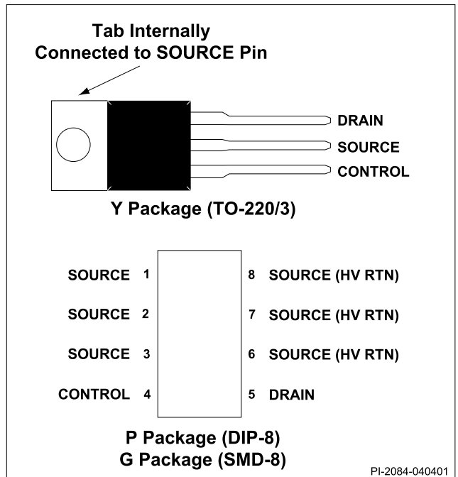
Figure 3. Pin Configuration.
