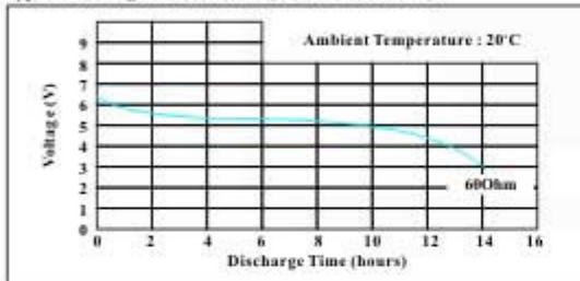
Typical Discharge Characteristics (Capacity vs. Loading)
