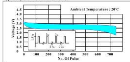
Typical Cycle Life (1.5A Pulse Drain)
