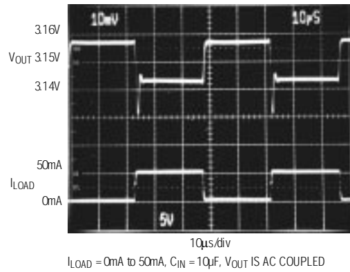
LOAD-TRANSIENT RESPONSE
