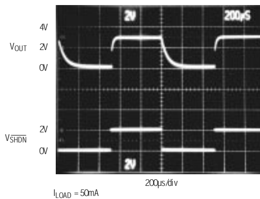
MAX8874 SHUTDOWN
