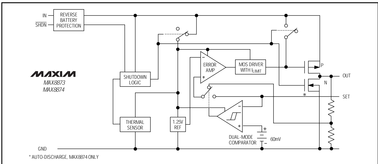
Figure 1. Functional Diagram
