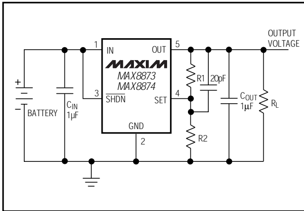
Figure 2 Adjustable Output Using External Feedback Resistors
