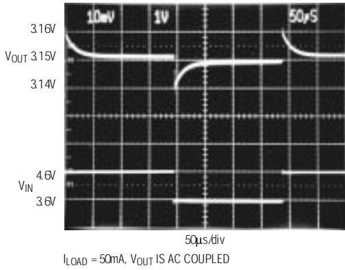
LINE-TRANSIENT RESPONSE
