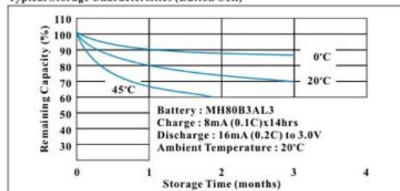
Typical Storage Characteristics (Button Cell)
