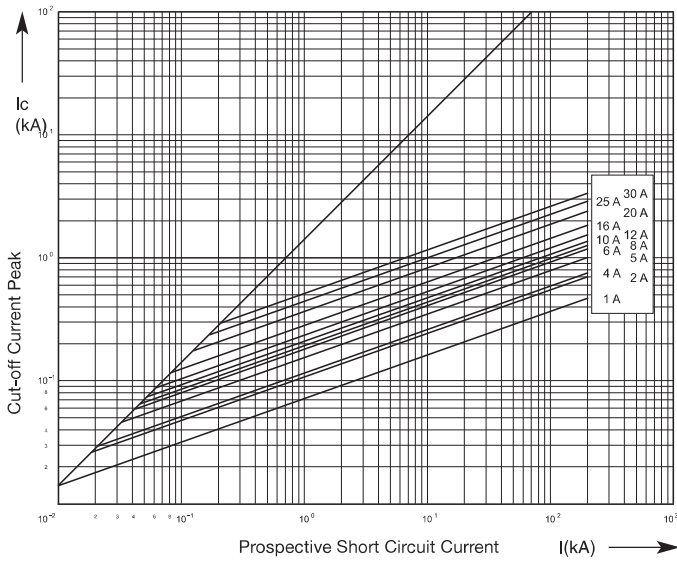
Cut-Off Characteristics
