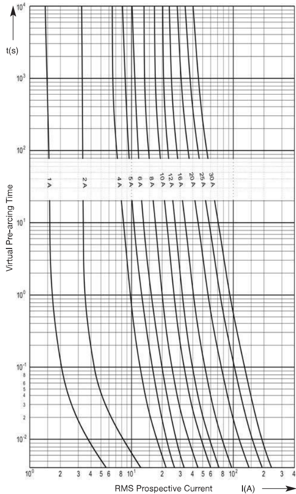
Time-Current Characteristics
