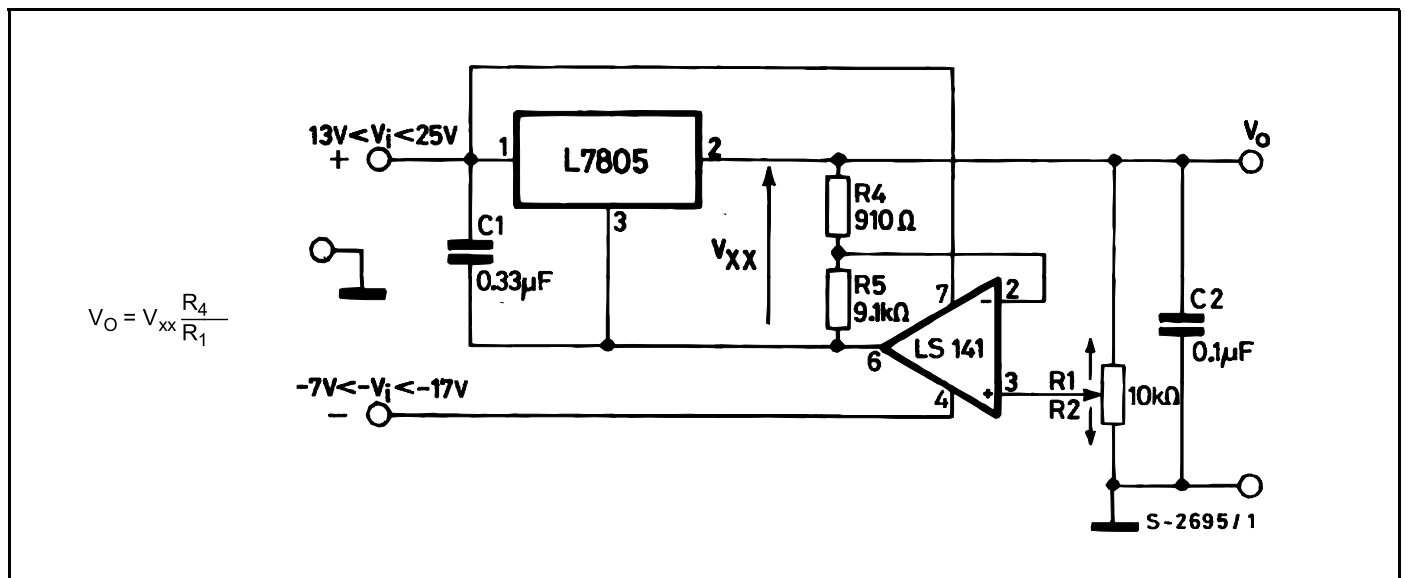
Figure 21: 0.5 to 10V Regulator
