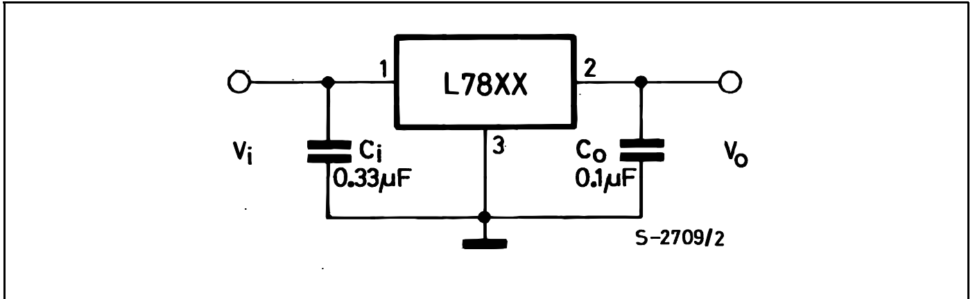
Figure 4: Application Circuits
