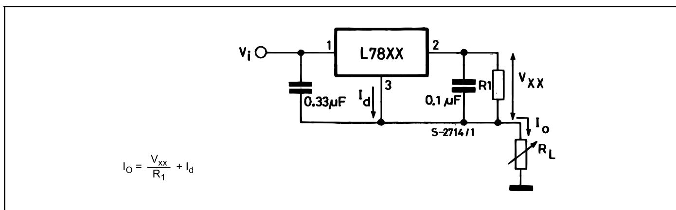
Figure 18: Current Regulator
