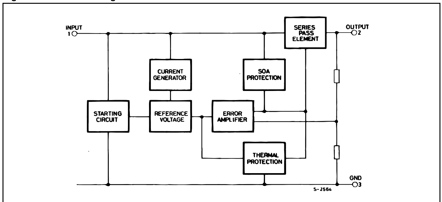
Figure 1: Schematic Diagram
