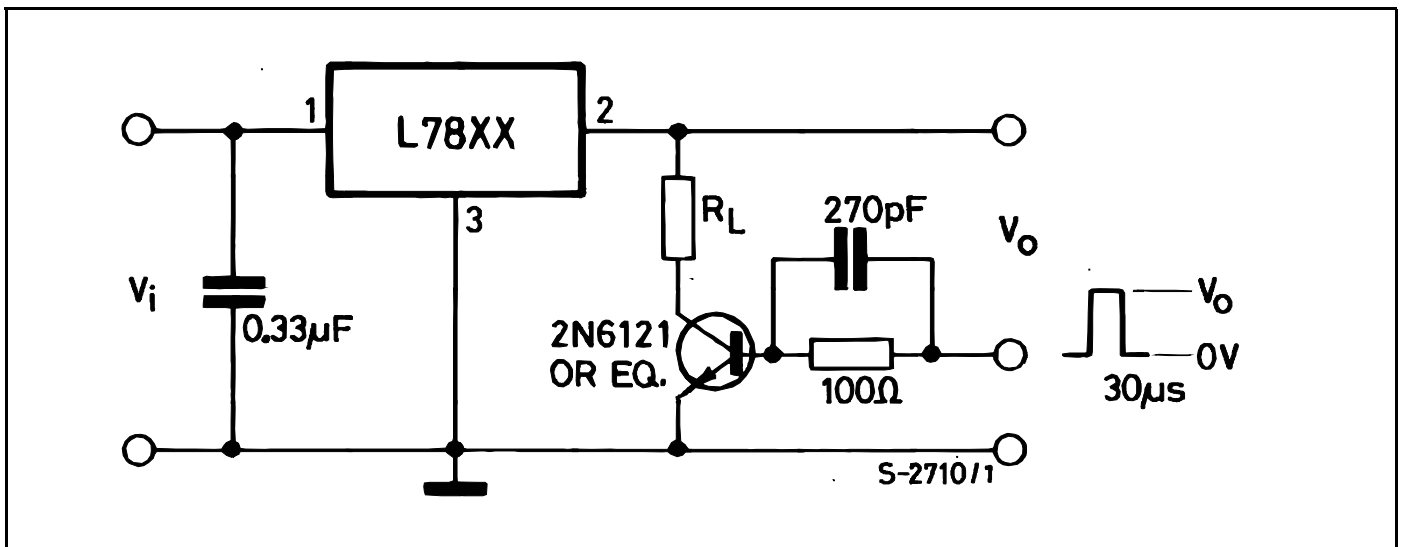
Figure 6: Load Regulation
