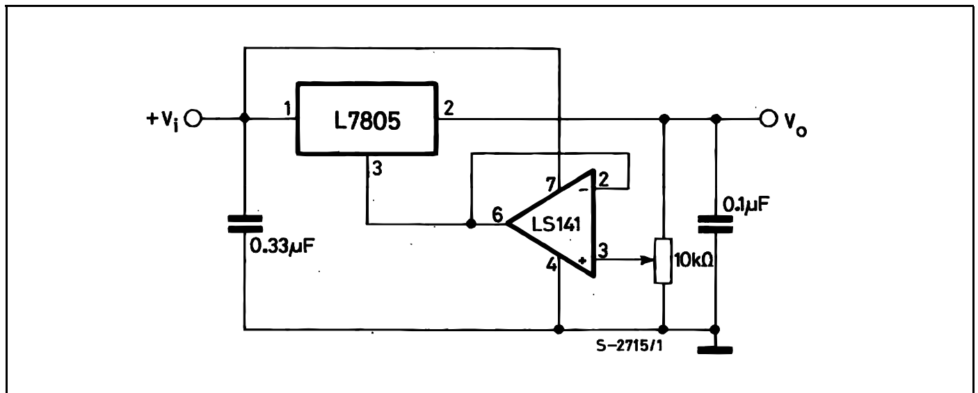
Figure 21: 0.5 to 10V Regulator
