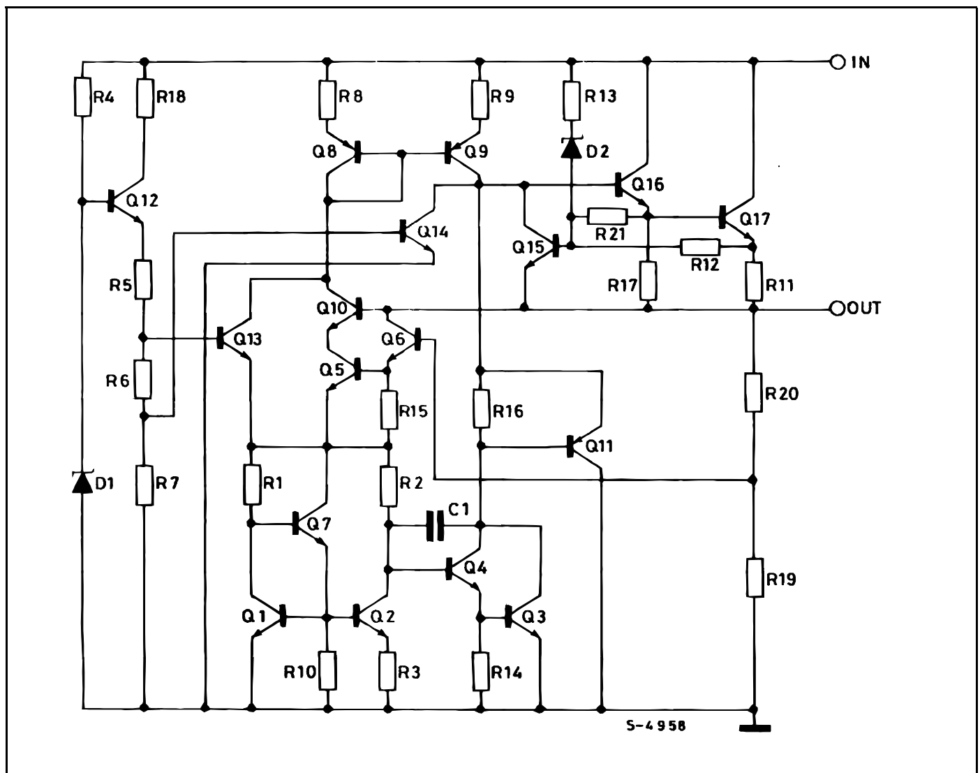
Figure 2: Schematic Diagram
