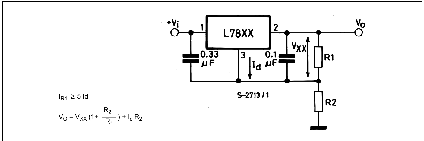
Figure 20: Adjustable Output Regulator (7 to 30V)
