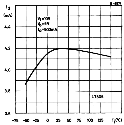
Figure 13: Quiescent Current vs Junction Temperature
