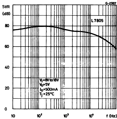
Figure 10: Supply Voltage Rejection vs Frequency
