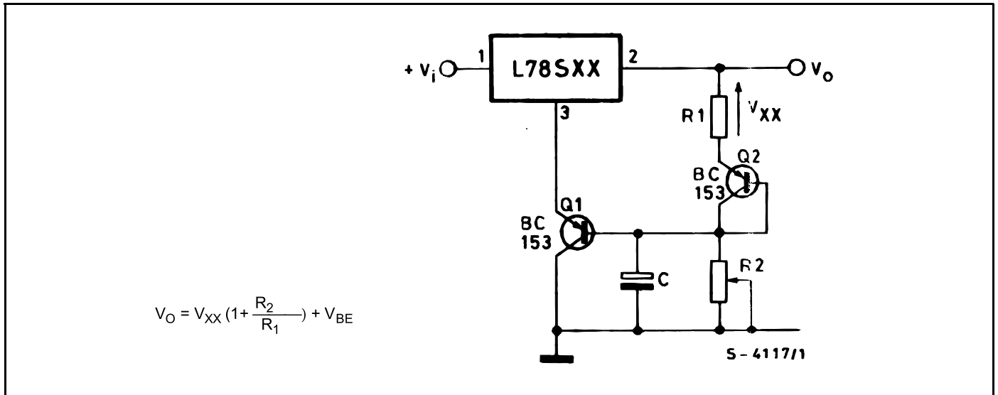
Figure 35: Adjustable Output Voltage with Temperature Compensation
