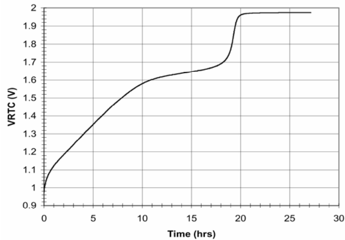
Charge characteristic
