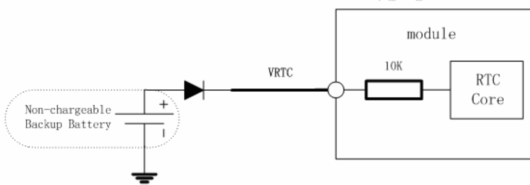
Figure 7: RTC supply from non-chargeable battery
