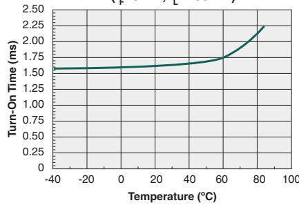
Typical Turn-On Time vs. Temperature ( I_F=3\text{mA}, I_L=100\text{mA} )
