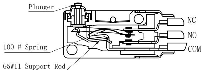
Internal structure digram
