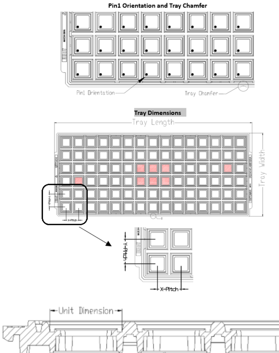
Figure 34. Tray Package Diagram
