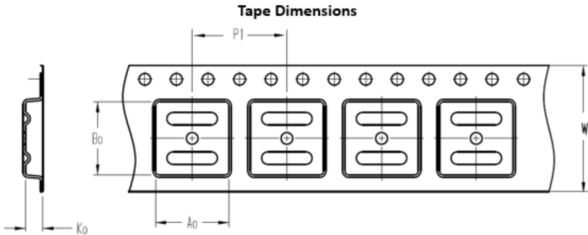
Figure 33. Strip Package Specification Diagram
