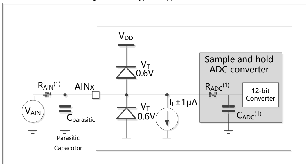
Figure 19. Typical application of ADC
