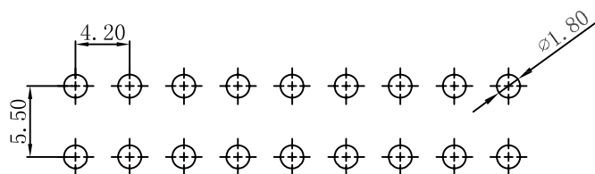
P. C. B LAYOUT
