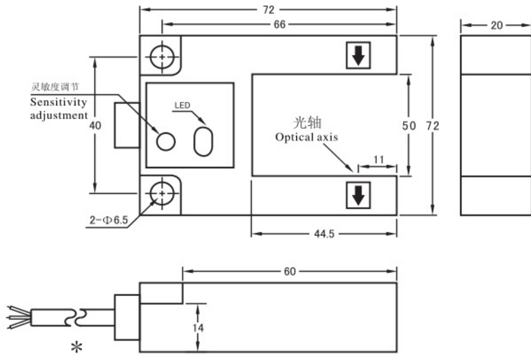
Chart 192 图192 E3S-GS50□
