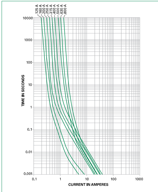
T-C Curves for 125mA to 800mA only
