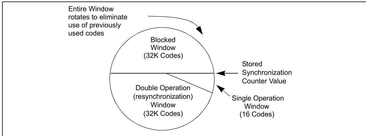
FIGURE 7-3: SYNCHRONIZATION WINDOW
