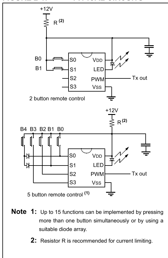
FIGURE 2-1: TYPICAL CIRCUITS
