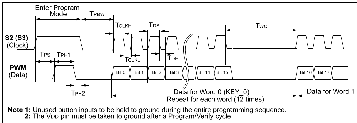
FIGURE 6-1: PROGRAMMING WAVEFORMS
