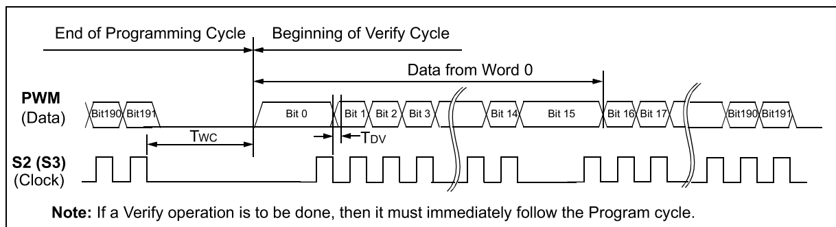
FIGURE 6-2: VERIFY WAVEFORMS
