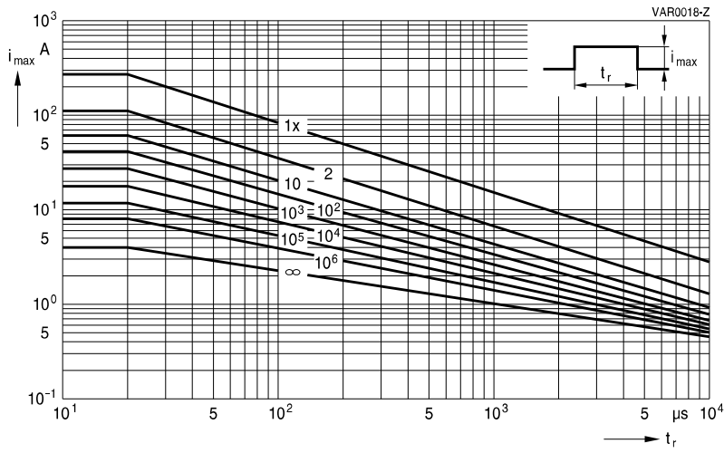
SIOV-S07K11 ... K40
