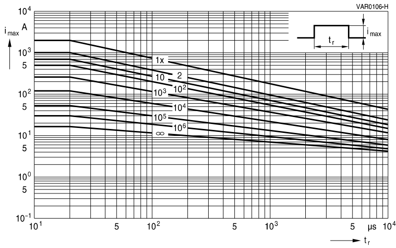
SIOV-S20K11 ... K40
