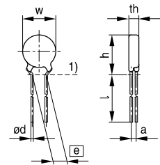
1) Seating plane to IEC 60717 VAR0412-N-E
