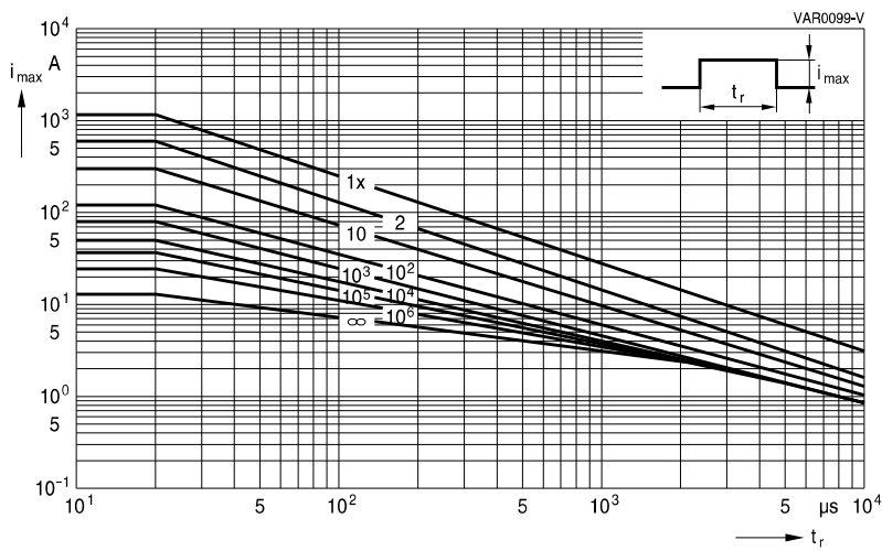
SIOV-S07K50 ... K460
