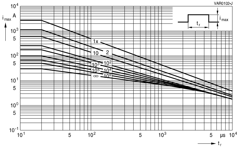
SIOV-S10K385 ... K680
