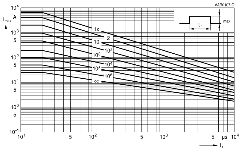
SIOV-S20K50 ... K115
