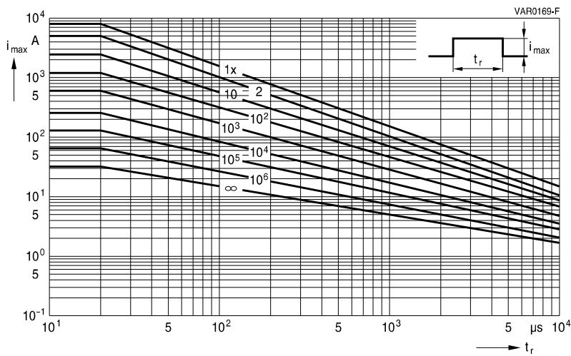
SIOV-S20K385 ... K460
