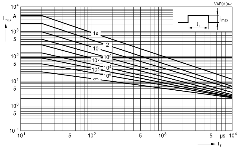
SIOV-S14K50 ... K320
