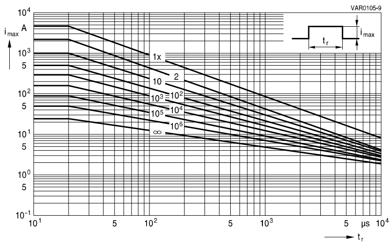
SIOV-S14K385 ... K1000
