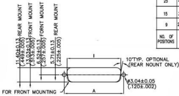
RECOMMENDED PANEL CUTOUT DIMENSIONS
