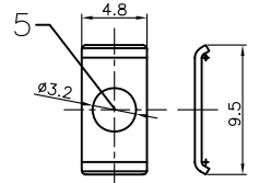
SMALL WASHER
