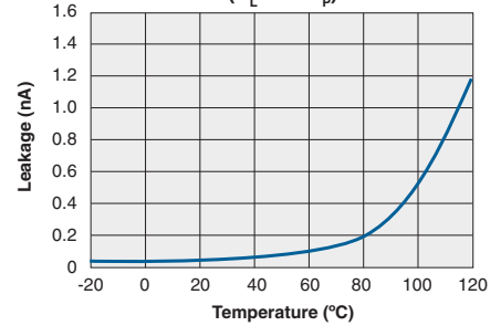
Typical Leakage vs. Temperature Measured Across Pins 3&4 ( V_L=100\text{V}_p )
