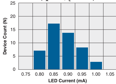
Typical I F for Switch Operation ( T_A=25^\circ\text{C} , I_L=100\text{mA} )
