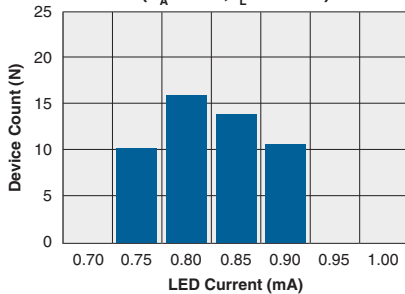
Typical I F for Switch Dropout ( T_A=25^\circ\text{C} , I_L=100\text{mA} )
