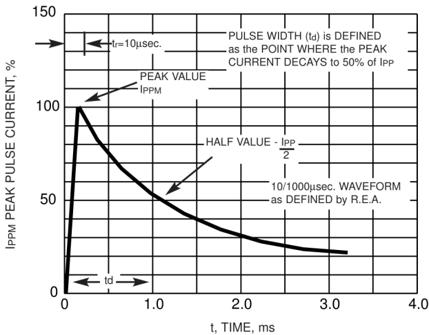
FIG. 3 - PULSE WAVEFORM
