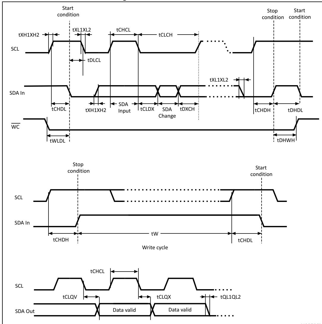
Figure 17. AC waveforms
