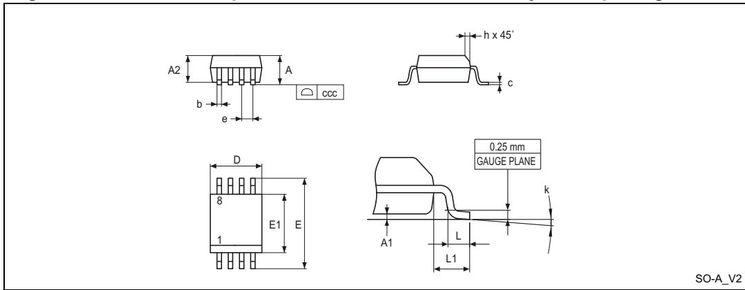
Figure 20. SO8N – 8-lead plastic small outline, 150 mils body width, package outline
