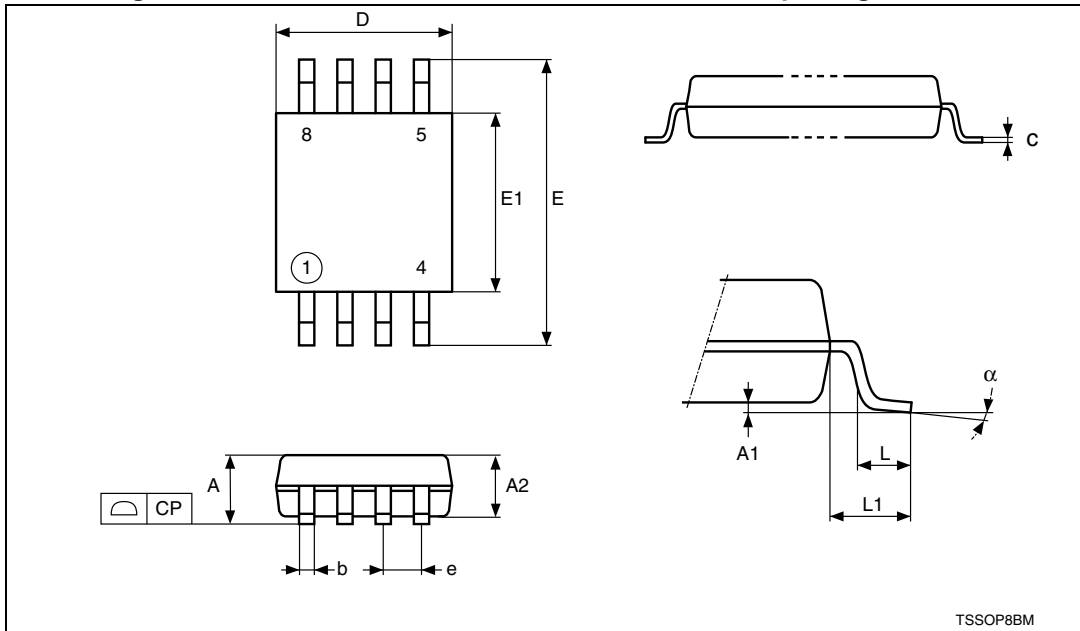
Figure 19. TSSOP8 – 8-lead thin shrink small outline, package outline
