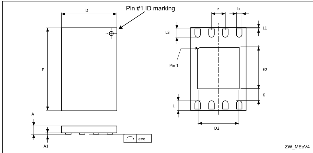
Figure 23. UFDFPN8 (MLP8) – 8-lead ultra thin fine pitch dual flat no lead, package outline
