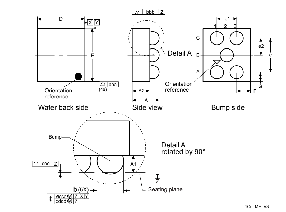
Figure 26. WLCSP 5-bump wafer-length chip-scale package outline (M24C64-FCS6TP/K)
