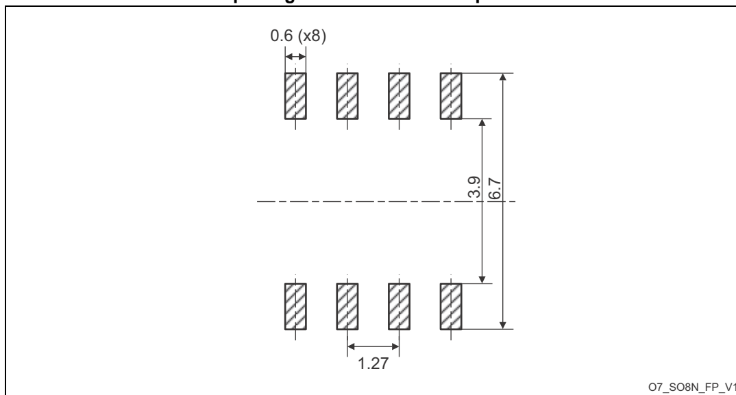
Figure 21. SO8N – 8-lead plastic small outline, 150 mils body width, package recommended footprint
