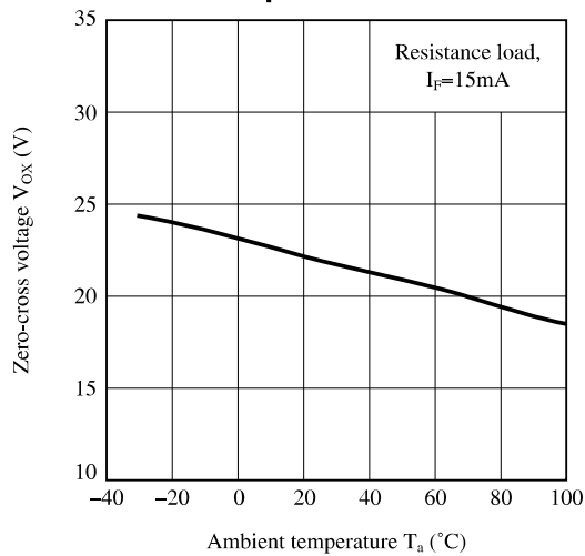
Fig.11 Zero-cross Voltage vs. Ambient Temperature
