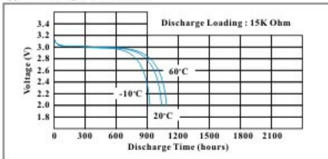
Typical Discharge Characteristics
