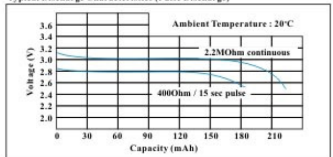
Typical Discharge Characteristics (Pulse Discharge)
