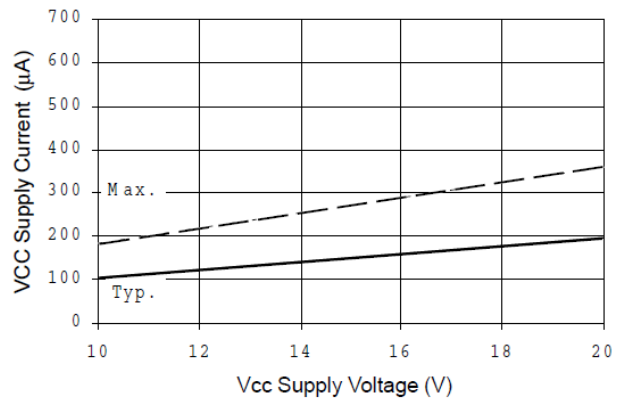
Figure 15B. V CC Supply Current vs. Voltage
