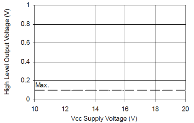
Figure 11B. High Level Output vs. Voltage
