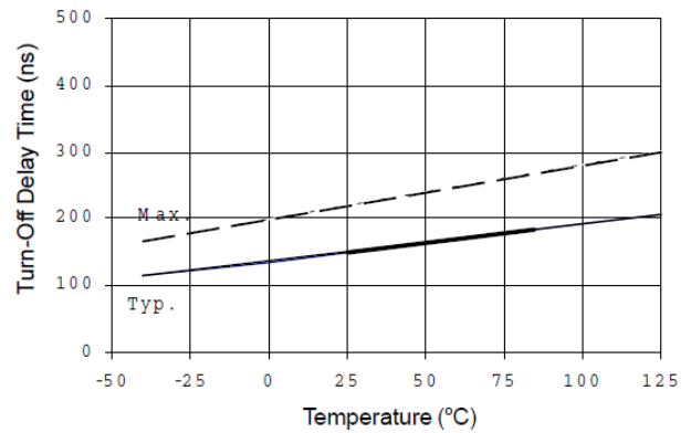
Figure 5A. Turn-Off Time vs. Temperature
