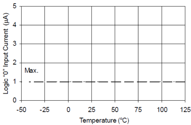
Figure 17A. Logic "0" Input Current vs. Temperature
