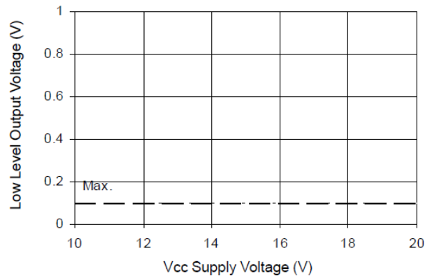
Figure 12B. Low Level Output vs. Voltage
