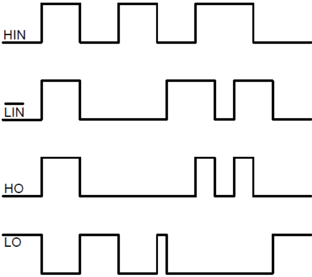
Figure 1. Input/Output Timing Diagram
