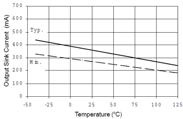
Figure 20A. Output Sink Current vs. Temperature
