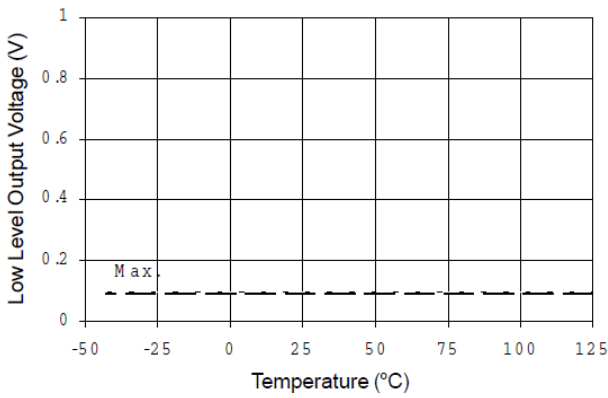
Figure 12A. Low Level Output vs. Temperature
