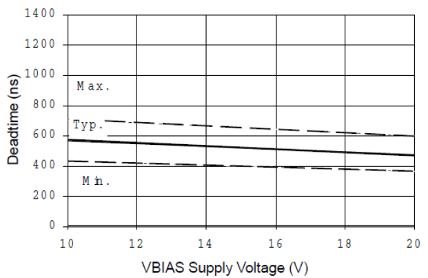
Figure 8B. Deadtime vs. Voltage
