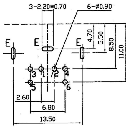
Pin Hole Layout (Jack Bottom View)
