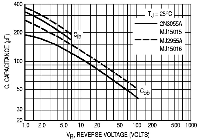
Figure 9. Capacitances
