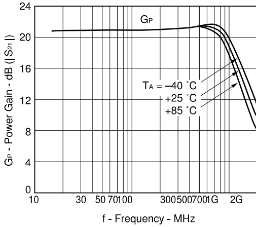
POWER GAIN ( |S_{21}| ) vs. FREQUENCY
