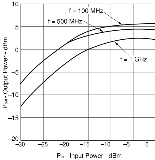
INPUT POWER vs. OUTPUT POWER
