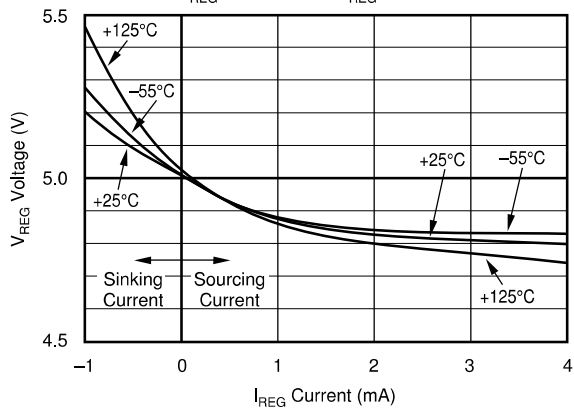
V_{REG} VOLTAGE vs V_{REG} CURRENT
