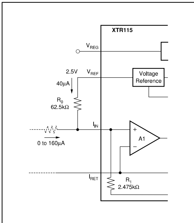
FIGURE 2. Creating Low-Scale Offset.
