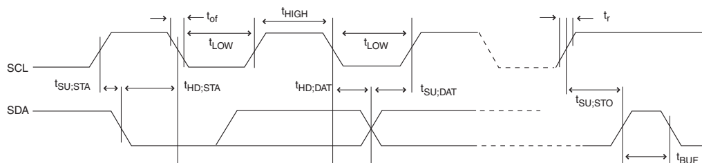
Figure 31-6. 2-wire Serial Bus Timing
