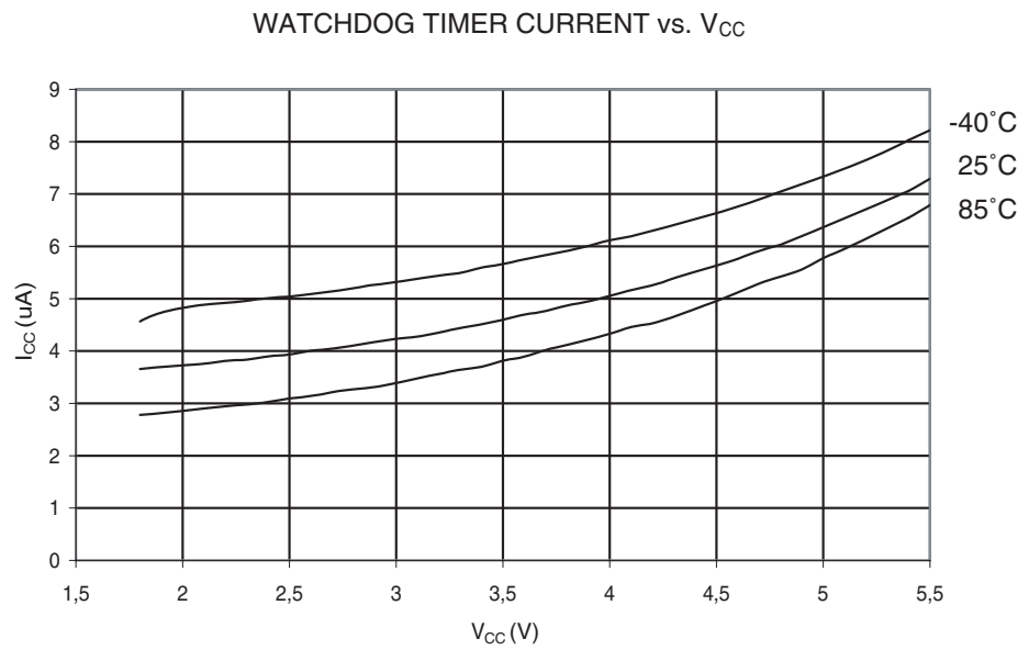
Figure 32-43. Watchdog Timer Current vs. V_{CC}
