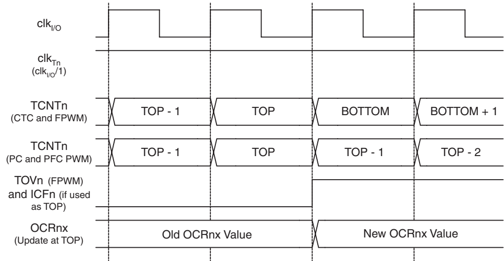
Figure 17-11. Timer/Counter Timing Diagram, no Prescaling
