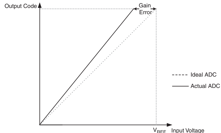
Figure 26-12. Gain Error
