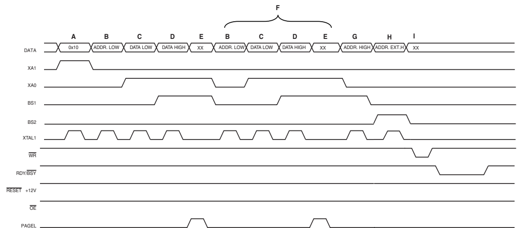
Figure 30-2. Programming the Flash Waveforms (1)
