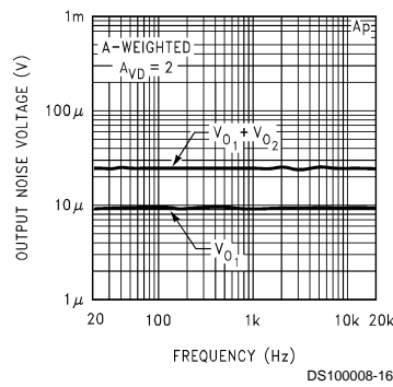
Noise Floor
