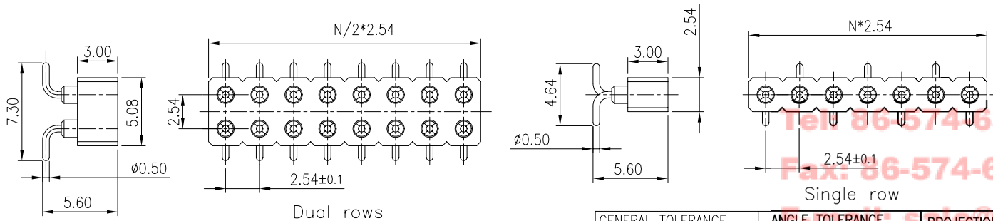
Dual rows Single row R/A TYPE
