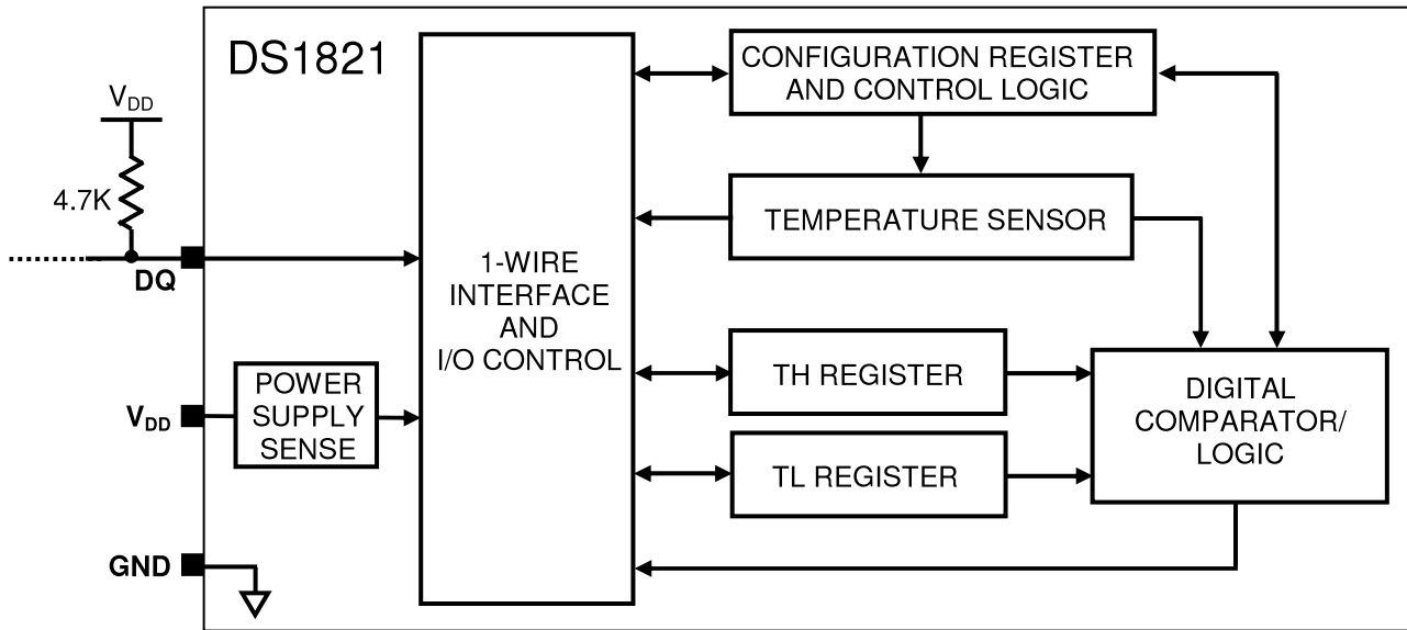
DS1821 BLOCK DIAGRAM Figure 1
