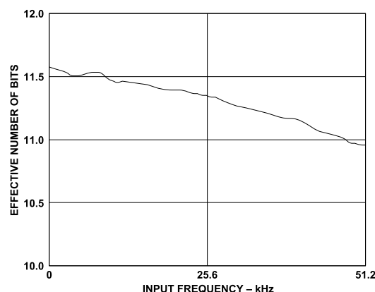
Figure 13. Effective Number of Bits vs. Frequency
