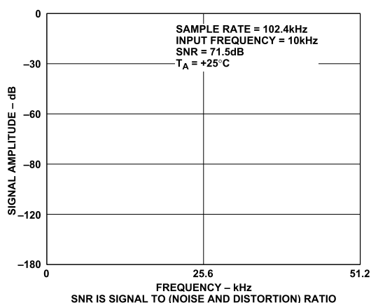
Figure 12. AD7893 FFT Plot
