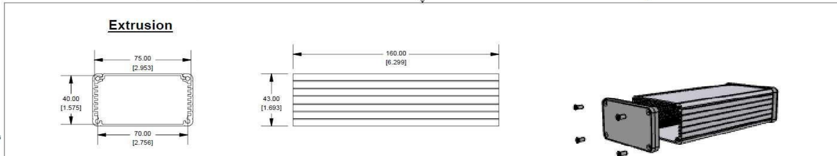
EXTRUSION DESIGNED FOR 75MM WIDE PC BOARD
