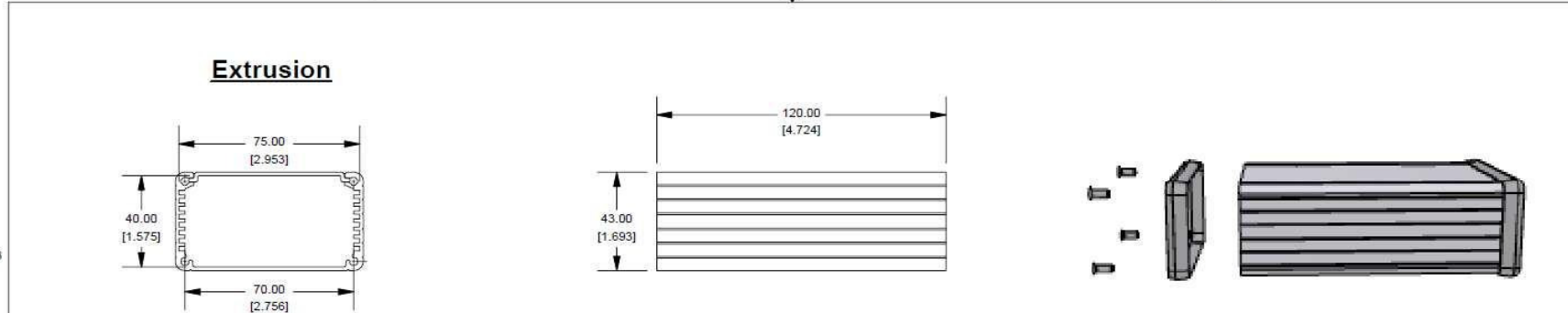
EXTRUSION DESIGNED FOR 75MM WIDE PC BOARD
